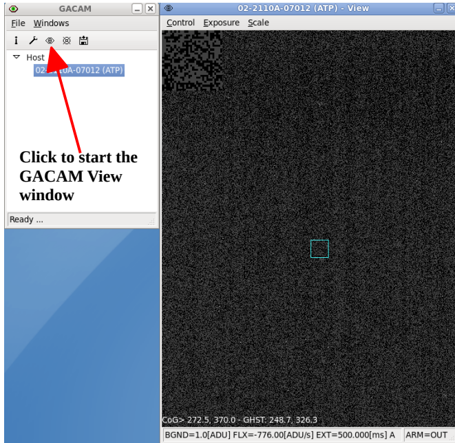
Figure 3. Left: ACAM GUI with camera live display window open
